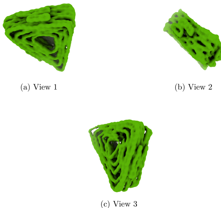
Figure 4: Isosurface at threshold=0.015400. Views generated by ChimeraX at a the following X, Y, Z angles: View 1 (0, -90, -90), View 2 (-90, 0, -90), View 3 (0, 0, 0).
