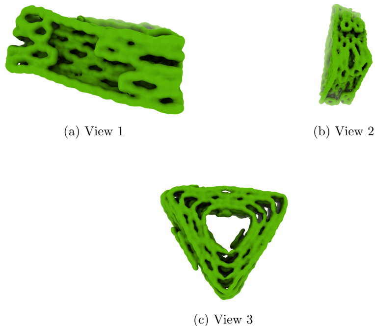
Figure 4: Isosurface at threshold=0.024700. Views generated by ChimeraX at a the following X, Y, Z angles: View 1 (0, -90, -90), View 2 (-90, 0, -90), View 3 (0, 0, 0).
