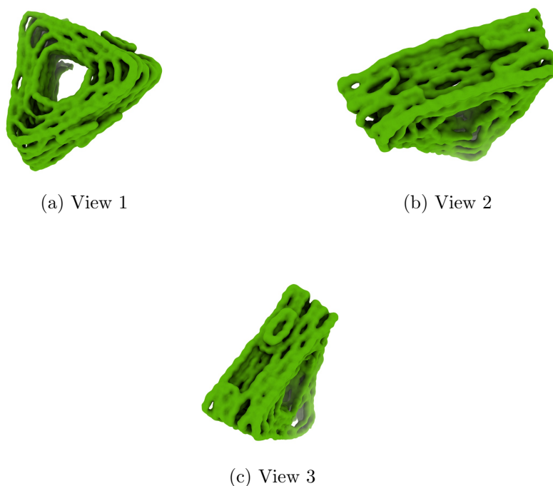
Figure 4: Isosurface at threshold=0.018800. Views generated by ChimeraX at a the following X, Y, Z angles: View 1 (0, -90, -90), View 2 (-90, 0, -90), View 3 (0, 0, 0).
