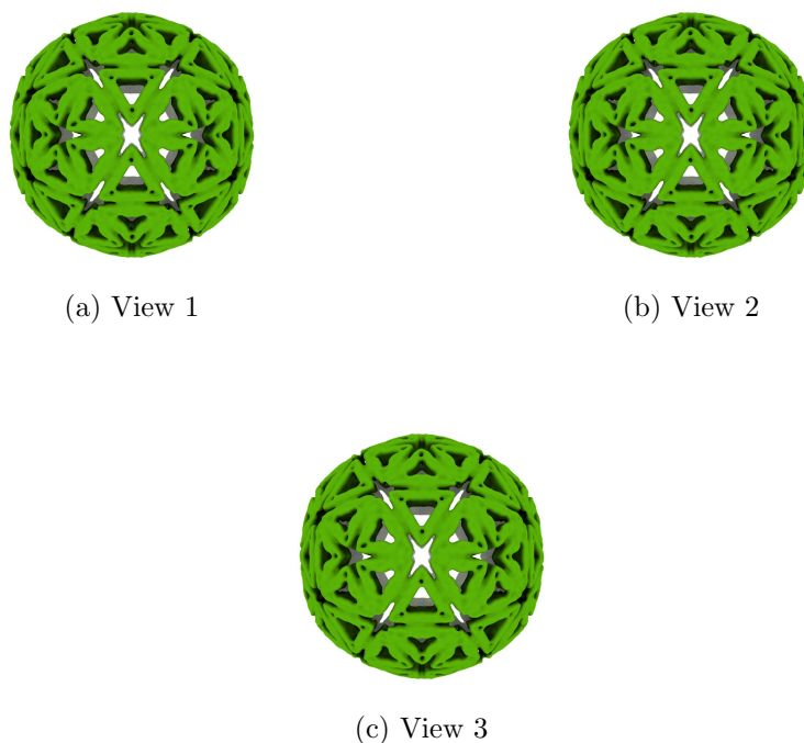
Figure 4: Isosurface at threshold=0.062200. Views generated by ChimeraX at a the following X, Y, Z angles: View 1 (0, -90, -90), View 2 (-90, 0, -90), View 3 (0, 0, 0).
