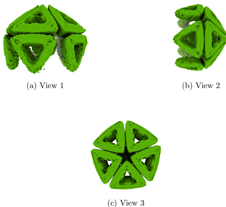
Figure 4: Isosurface at threshold=0.067300. Views generated by ChimeraX at a the following X, Y, Z angles: View 1 (0, -90, -90), View 2 (-90, 0, -90), View 3 (0, 0, 0).
