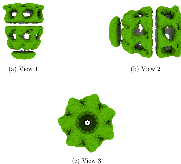
Figure 4: Isosurface at threshold=0.749000. Views generated by ChimeraX at a the following X, Y, Z angles: View 1 (0, -90, -90), View 2 (-90, 0, -90), View 3 (0, 0, 0).
