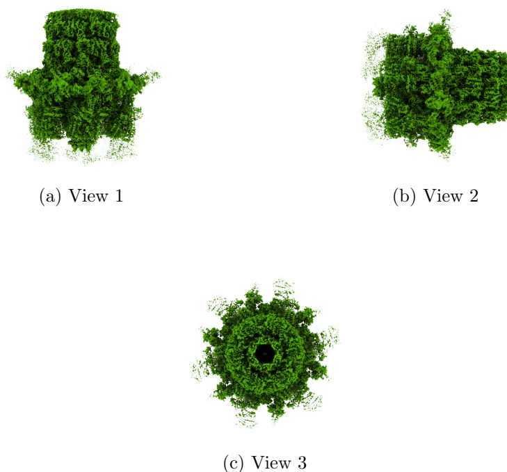
Figure 4: Isosurface at threshold=0.030900. Views generated by ChimeraX at a the following X, Y, Z angles: View 1 (0, -90, -90), View 2 (-90, 0, -90), View 3 (0, 0, 0).
