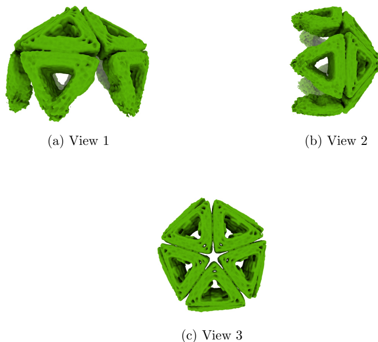
Figure 4: Isosurface at threshold=0.028300. Views generated by ChimeraX at a the following X, Y, Z angles: View 1 (0, -90, -90), View 2 (-90, 0, -90), View 3 (0, 0, 0).
