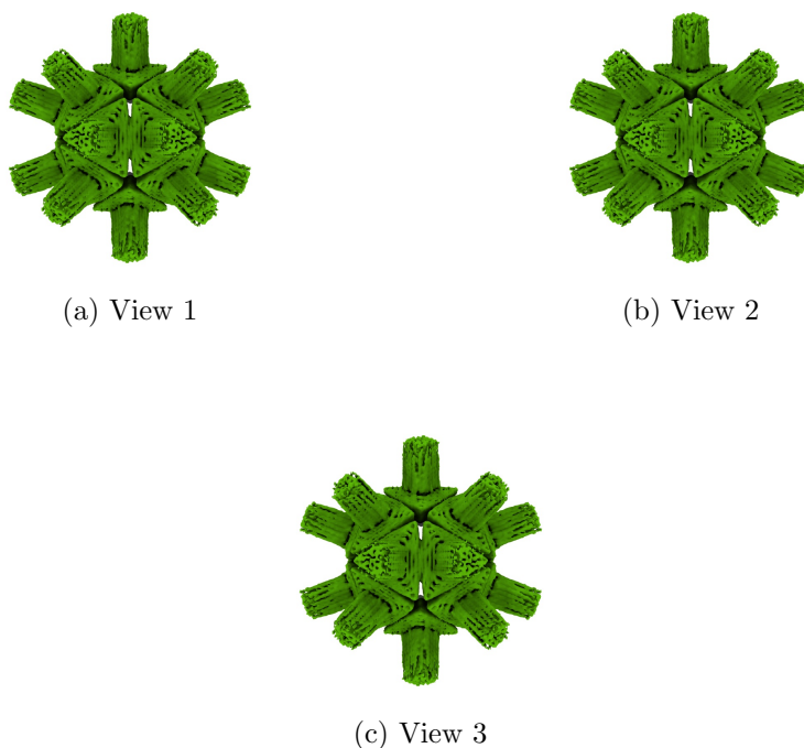
Figure 4: Isosurface at threshold=0.002540. Views generated by ChimeraX at a the following X, Y, Z angles: View 1 (0, -90, -90), View 2 (-90, 0, -90), View 3 (0, 0, 0).
