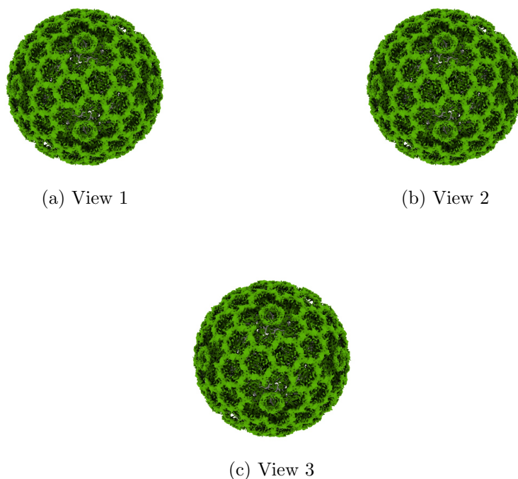
Figure 4: Isosurface at threshold=1800.000000. Views generated by ChimeraX at the following X, Y, Z angles: View 1 (0, -90, -90), View 2 (-90, 0, -90), View 3 (0, 0, 0).
