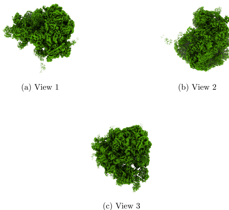
Figure 4: Isosurface at threshold=0.035600. Views generated by ChimeraX at a the following X, Y, Z angles: View 1 (0, -90, -90), View 2 (-90, 0, -90), View 3 (0, 0, 0).
