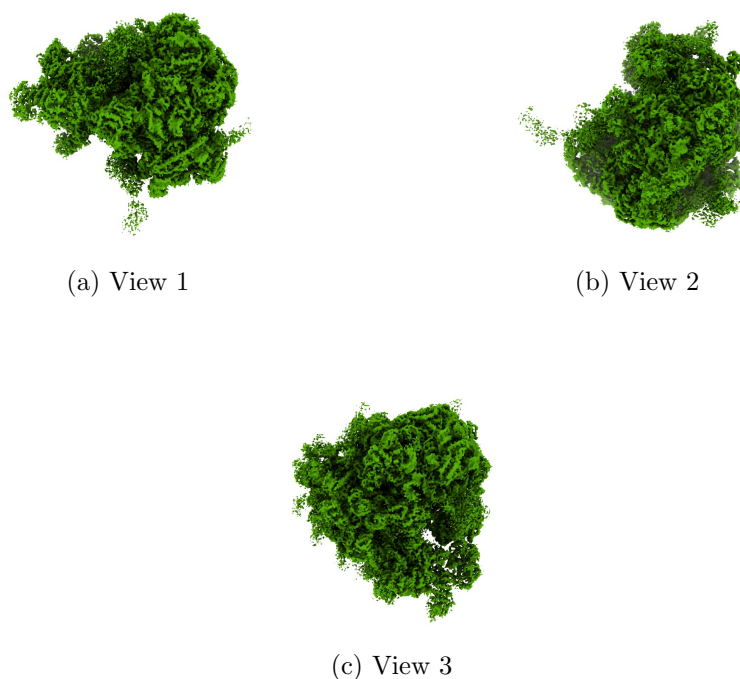
Figure 4: Isosurface at threshold=0.031600. Views generated by ChimeraX at a the following X, Y, Z angles: View 1 (0, -90, -90), View 2 (-90, 0, -90), View 3 (0, 0, 0).
