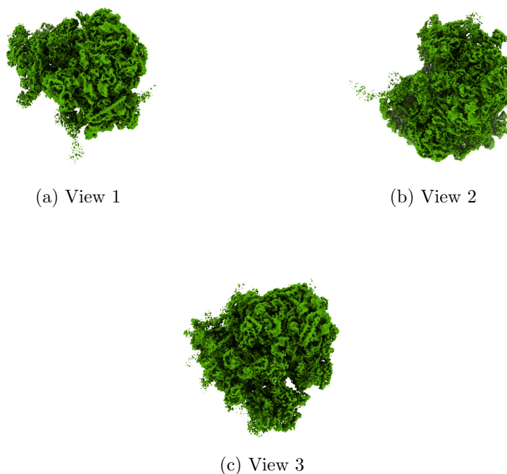
Figure 4: Isosurface at threshold=0.030800. Views generated by ChimeraX at a the following X, Y, Z angles: View 1 (0, -90, -90), View 2 (-90, 0, -90), View 3 (0, 0, 0).
