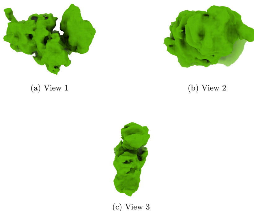
Figure 4: Isosurface at threshold=0.049400. Views generated by ChimeraX at a the following X, Y, Z angles: View 1 (0, -90, -90), View 2 (-90, 0, -90), View 3 (0, 0, 0).
