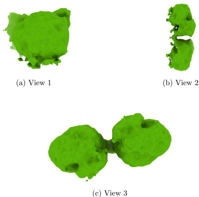
Figure 4: Isosurface at threshold=1.190000. Views generated by ChimeraX at a the following X, Y, Z angles: View 1 (0, -90, -90), View 2 (-90, 0, -90), View 3 (0, 0, 0).
