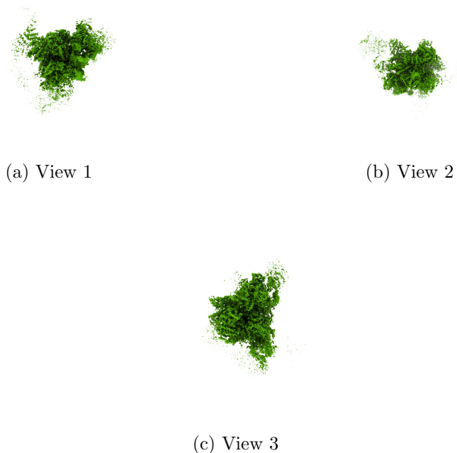
Figure 4: Isosurface at threshold=0.019000. Views generated by ChimeraX at a the following X, Y, Z angles: View 1 (0, -90, -90), View 2 (-90, 0, -90), View 3 (0, 0, 0).
