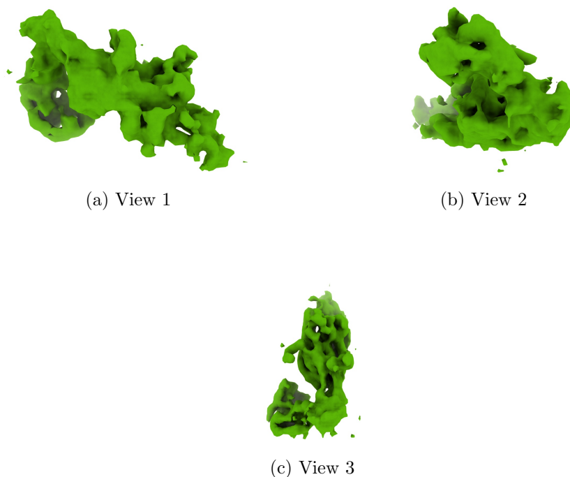
Figure 4: Isosurface at threshold=0.013000. Views generated by ChimeraX at a the following X, Y, Z angles: View 1 (0, -90, -90), View 2 (-90, 0, -90), View 3 (0, 0, 0).
