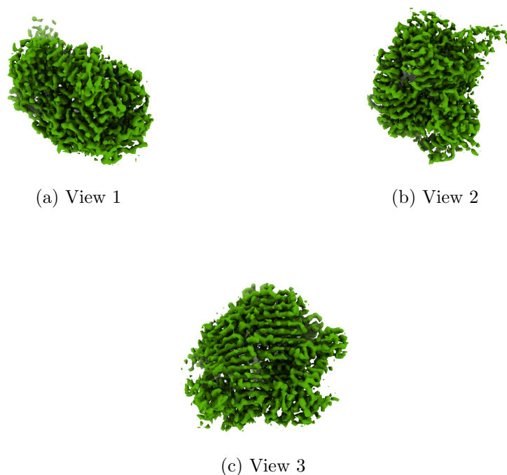
Figure 4: Isosurface at threshold=0.073000. Views generated by ChimeraX at a the following X, Y, Z angles: View 1 (0, -90, -90), View 2 (-90, 0, -90), View 3 (0, 0, 0).
