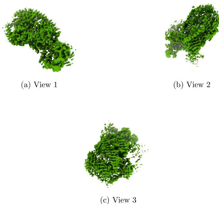
Figure 4: Isosurface at threshold=0.098000. Views generated by ChimeraX at a the following X, Y, Z angles: View 1 (0, -90, -90), View 2 (-90, 0, -90), View 3 (0, 0, 0).
