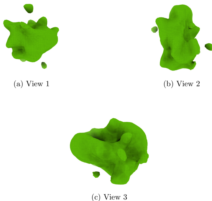
Figure 4: Isosurface at threshold=1.880000. Views generated by ChimeraX at a the following X, Y, Z angles: View 1 (0, -90, -90), View 2 (-90, 0, -90), View 3 (0, 0, 0).
