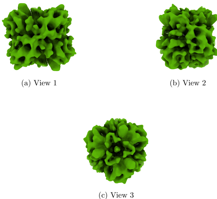
Figure 4: Isosurface at threshold=0.003600. Views generated by ChimeraX at a the following X, Y, Z angles: View 1 (0, -90, -90), View 2 (-90, 0, -90), View 3 (0, 0, 0).
