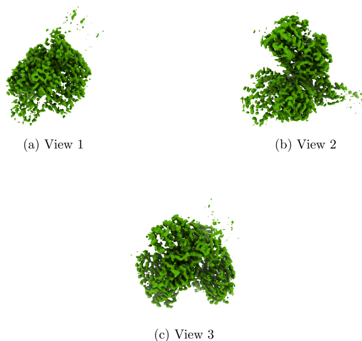
Figure 4: Isosurface at threshold=0.017400. Views generated by ChimeraX at a the following X, Y, Z angles: View 1 (0, -90, -90), View 2 (-90, 0, -90), View 3 (0, 0, 0).
