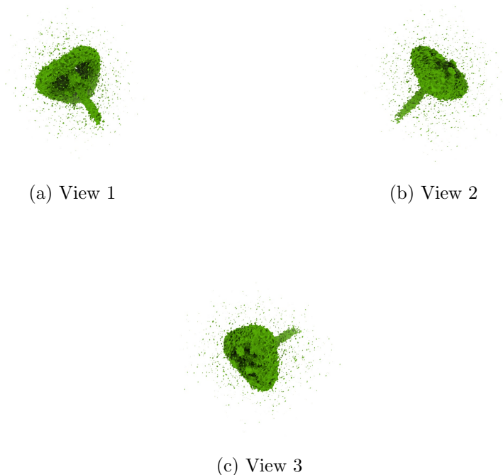
Figure 4: Isosurface at threshold=0.019100. Views generated by ChimeraX at a the following X, Y, Z angles: View 1 (0, -90, -90), View 2 (-90, 0, -90), View 3 (0, 0, 0).
