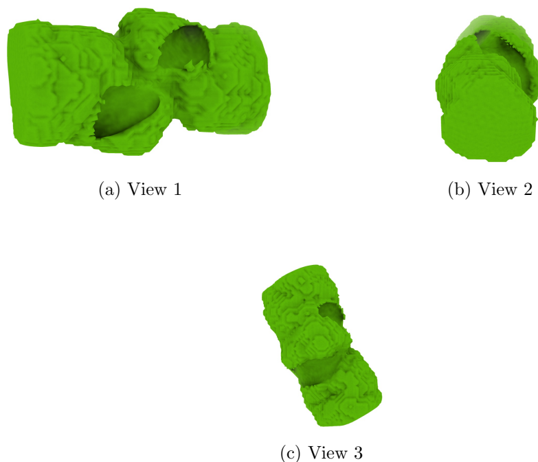
Figure 4: Isosurface at threshold=14.100000. Views generated by ChimeraX at a the following X, Y, Z angles: View 1 (0, -90, -90), View 2 (-90, 0, -90), View 3 (0, 0, 0).
