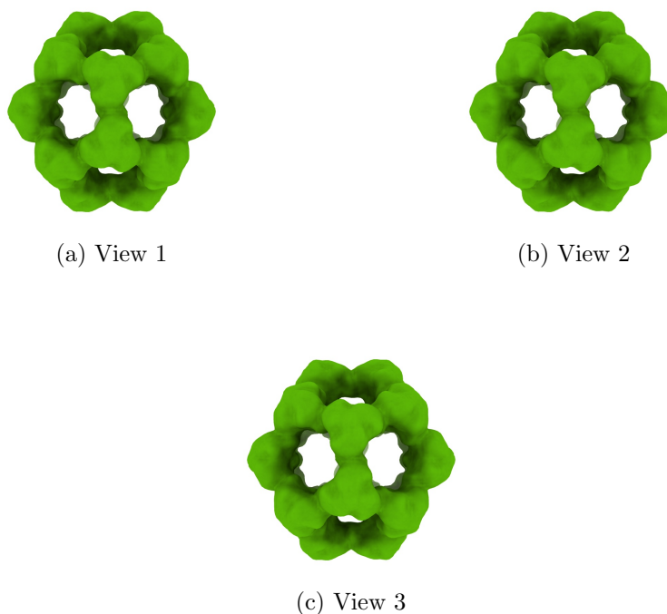
Figure 4: Isosurface at threshold=0.074700. Views generated by ChimeraX at a the following X, Y, Z angles: View 1 (0, -90, -90), View 2 (-90, 0, -90), View 3 (0, 0, 0).
