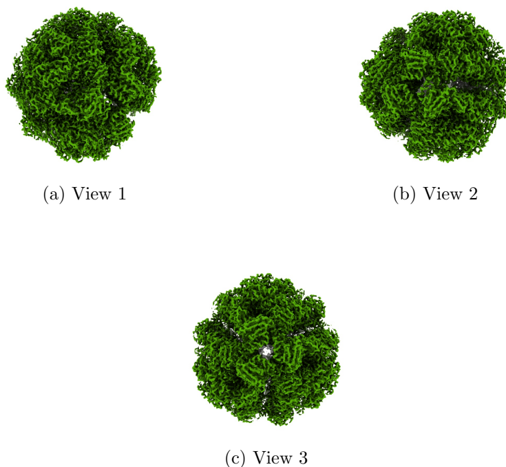
Figure 4: Isosurface at threshold=0.028700. Views generated by ChimeraX at a the following X, Y, Z angles: View 1 (0, -90, -90), View 2 (-90, 0, -90), View 3 (0, 0, 0).
