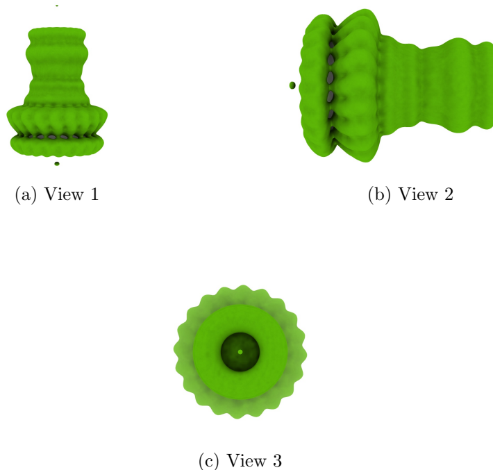
Figure 4: Isosurface at threshold=0.034600. Views generated by ChimeraX at the following X, Y, Z angles: View 1 (0, -90, -90), View 2 (-90, 0, -90), View 3 (0, 0, 0).
