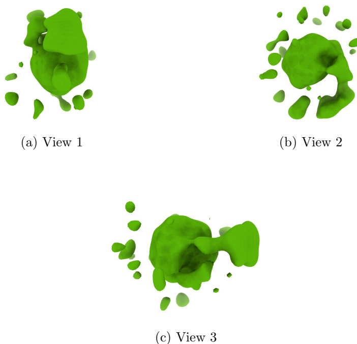
Figure 4: Isosurface at threshold=1.240000. Views generated by ChimeraX at a the following X, Y, Z angles: View 1 (0, -90, -90), View 2 (-90, 0, -90), View 3 (0, 0, 0).
