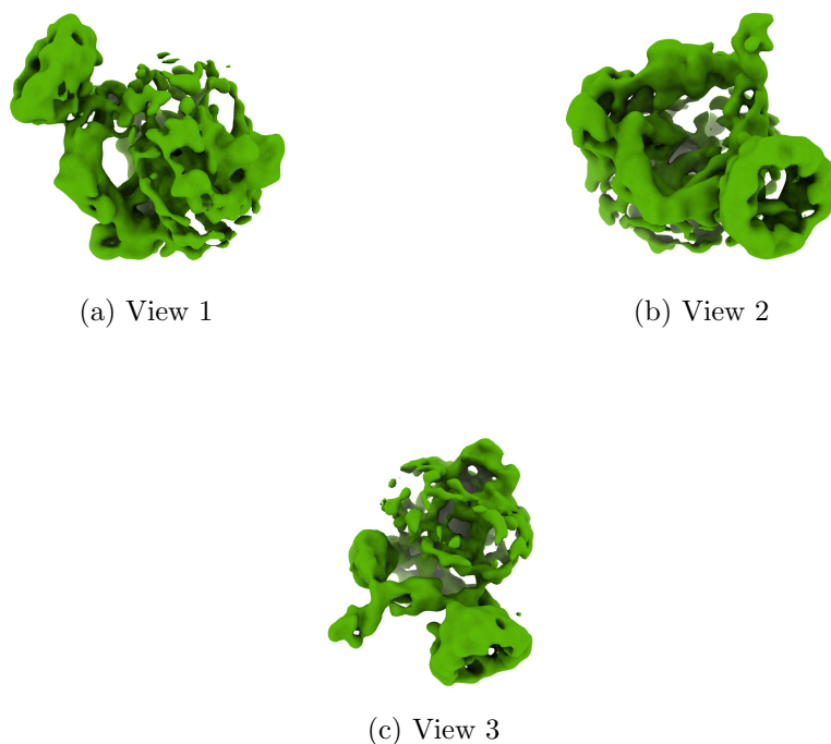
Figure 4: Isosurface at threshold=0.007320. Views generated by ChimeraX at a the following X, Y, Z angles: View 1 (0, -90, -90), View 2 (-90, 0, -90), View 3 (0, 0, 0).
