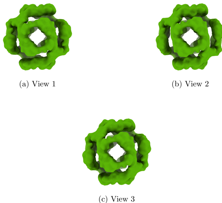
Figure 4: Isosurface at threshold=0.025400. Views generated by ChimeraX at a the following X, Y, Z angles: View 1 (0, -90, -90), View 2 (-90, 0, -90), View 3 (0, 0, 0).
