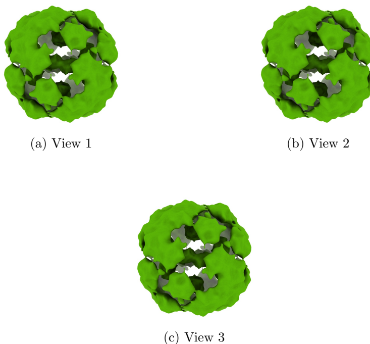
Figure 4: Isosurface at threshold=0.026300. Views generated by ChimeraX at the following X, Y, Z angles: View 1 (0, -90, -90), View 2 (-90, 0, -90), View 3 (0, 0, 0).
