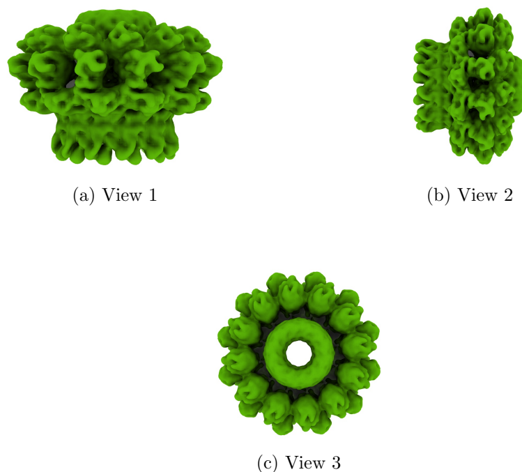
Figure 4: Isosurface at threshold=0.371000. Views generated by ChimeraX at a the following X, Y, Z angles: View 1 (0, -90, -90), View 2 (-90, 0, -90), View 3 (0, 0, 0).
