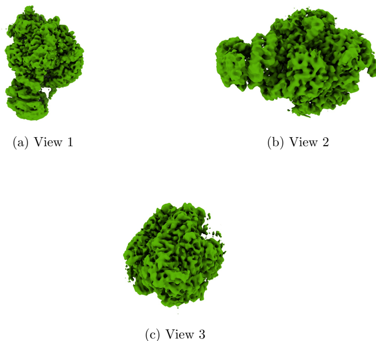
Figure 4: Isosurface at threshold=0.050500. Views generated by ChimeraX at a the following X, Y, Z angles: View 1 (0, -90, -90), View 2 (-90, 0, -90), View 3 (0, 0, 0).
