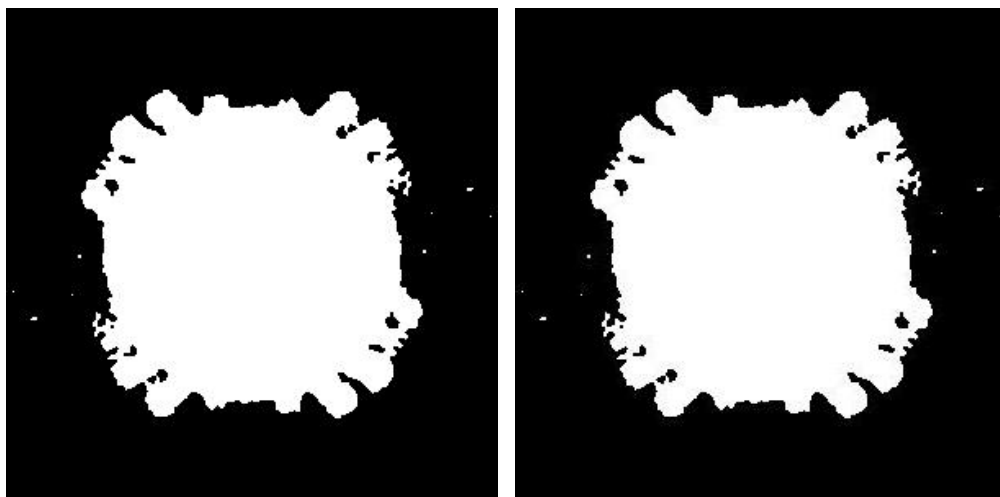
(a) X Slice 147
