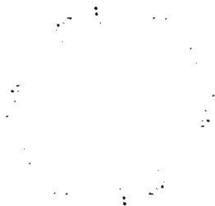
(c) Z Slice 132
