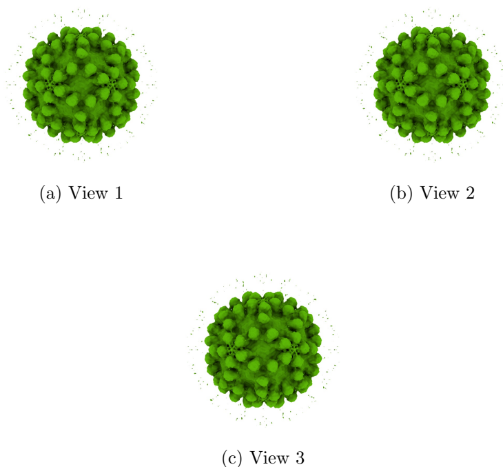
Figure 4: Isosurface at threshold=611.000000. Views generated by ChimeraX at a the following X, Y, Z angles: View 1 (0, -90, -90), View 2 (-90, 0, -90), View 3 (0, 0, 0).
