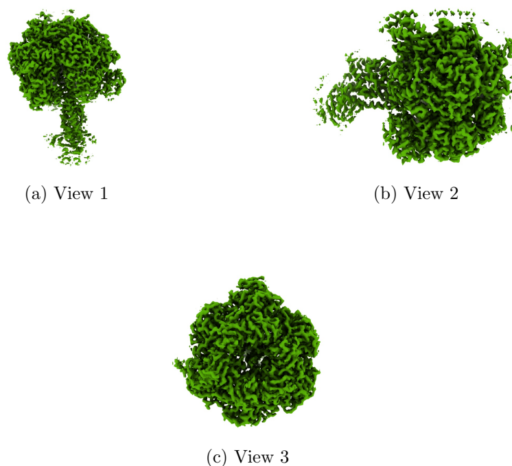
Figure 4: Isosurface at threshold=0.018100. Views generated by ChimeraX at a the following X, Y, Z angles: View 1 (0, -90, -90), View 2 (-90, 0, -90), View 3 (0, 0, 0).
