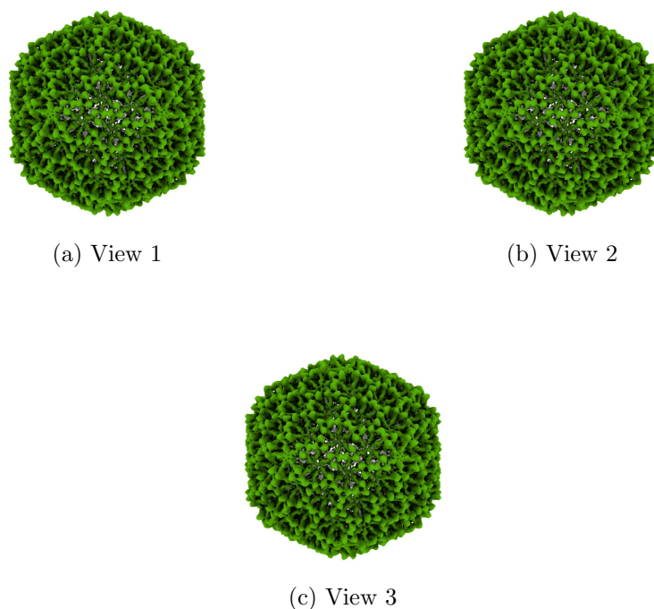
Figure 4: Isosurface at threshold=3.220000. Views generated by ChimeraX at a the following X, Y, Z angles: View 1 (0, -90, -90), View 2 (-90, 0, -90), View 3 (0, 0, 0).
