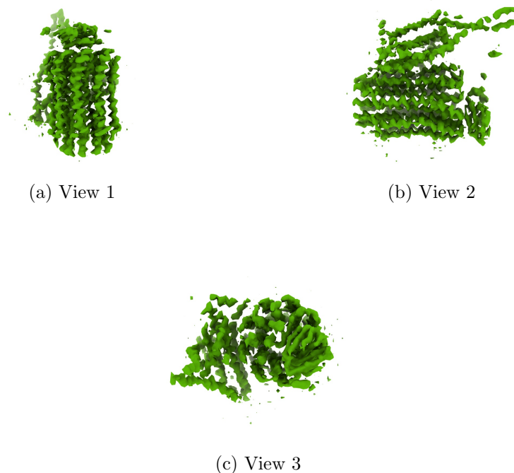
Figure 4: Isosurface at threshold=0.015400. Views generated by ChimeraX at a the following X, Y, Z angles: View 1 (0, -90, -90), View 2 (-90, 0, -90), View 3 (0, 0, 0).
