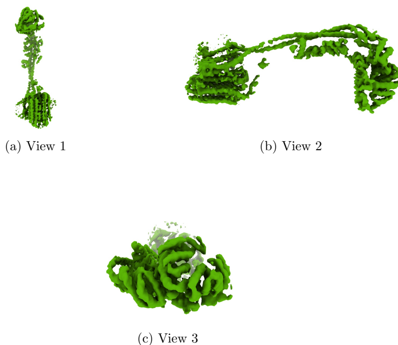
Figure 4: Isosurface at threshold=0.010900. Views generated by ChimeraX at a the following X, Y, Z angles: View 1 (0, -90, -90), View 2 (-90, 0, -90), View 3 (0, 0, 0).
