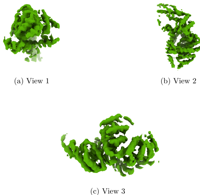
Figure 4: Isosurface at threshold=0.013500. Views generated by ChimeraX at a the following X, Y, Z angles: View 1 (0, -90, -90), View 2 (-90, 0, -90), View 3 (0, 0, 0).
