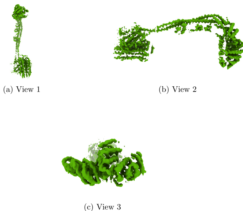
Figure 4: Isosurface at threshold=0.013500. Views generated by ChimeraX at a the following X, Y, Z angles: View 1 (0, -90, -90), View 2 (-90, 0, -90), View 3 (0, 0, 0).
