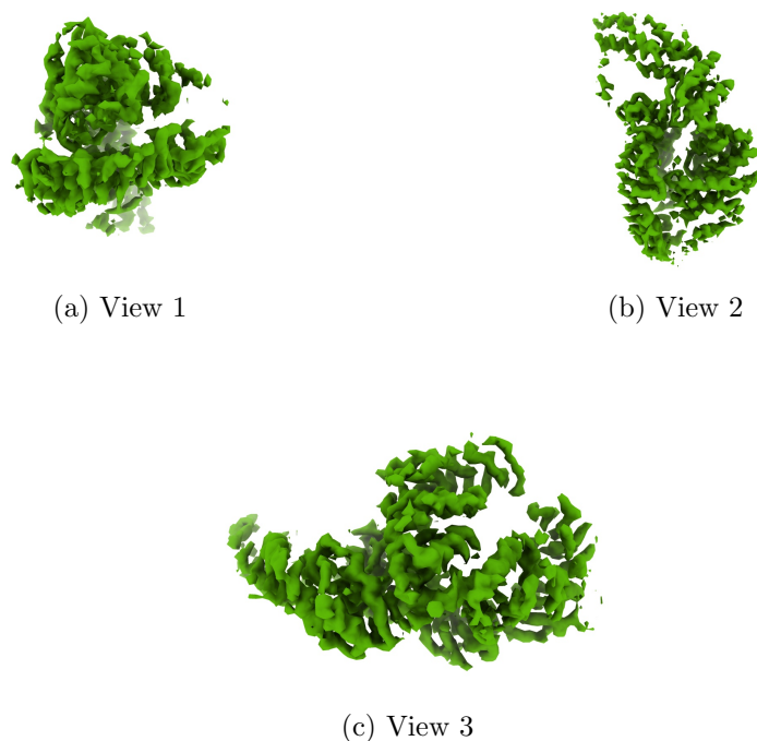
Figure 4: Isosurface at threshold=0.017200. Views generated by ChimeraX at a the following X, Y, Z angles: View 1 (0, -90, -90), View 2 (-90, 0, -90), View 3 (0, 0, 0).
