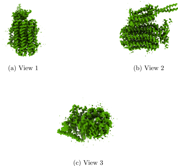
Figure 4: Isosurface at threshold=0.016900. Views generated by ChimeraX at a the following X, Y, Z angles: View 1 (0, -90, -90), View 2 (-90, 0, -90), View 3 (0, 0, 0).
