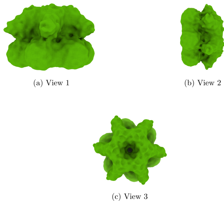
Figure 4: Isosurface at threshold=0.920000. Views generated by ChimeraX at a the following X, Y, Z angles: View 1 (0, -90, -90), View 2 (-90, 0, -90), View 3 (0, 0, 0).
