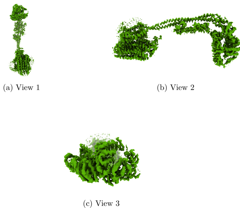
Figure 4: Isosurface at threshold=0.012800. Views generated by ChimeraX at a the following X, Y, Z angles: View 1 (0, -90, -90), View 2 (-90, 0, -90), View 3 (0, 0, 0).
