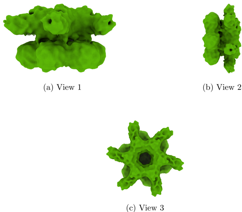
Figure 4: Isosurface at threshold=0.956000. Views generated by ChimeraX at a the following X, Y, Z angles: View 1 (0, -90, -90), View 2 (-90, 0, -90), View 3 (0, 0, 0).
