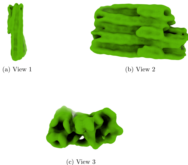
Figure 4: Isosurface at threshold=0.045400. Views generated by ChimeraX at a the following X, Y, Z angles: View 1 (0, -90, -90), View 2 (-90, 0, -90), View 3 (0, 0, 0).
