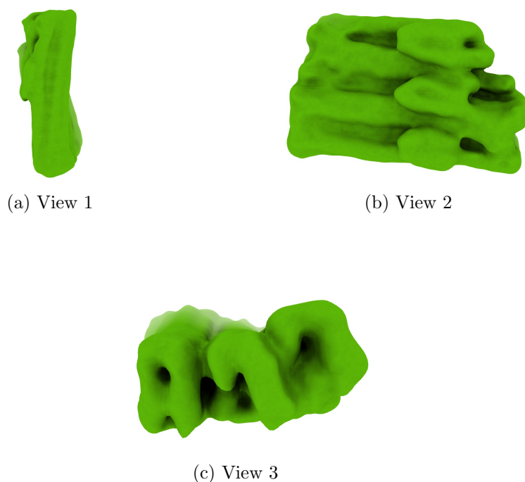
Figure 4: Isosurface at threshold=0.017800. Views generated by ChimeraX at a the following X, Y, Z angles: View 1 (0, -90, -90), View 2 (-90, 0, -90), View 3 (0, 0, 0).
