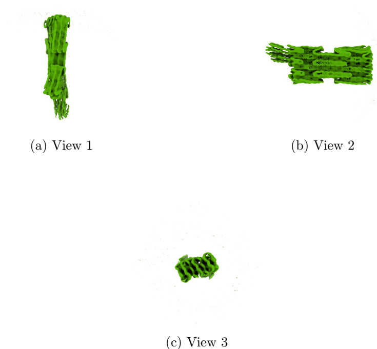
Figure 4: Isosurface at threshold=0.244000. Views generated by ChimeraX at a the following X, Y, Z angles: View 1 (0, -90, -90), View 2 (-90, 0, -90), View 3 (0, 0, 0).
