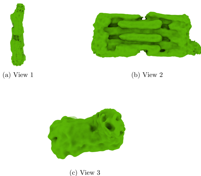
Figure 4: Isosurface at threshold=0.029900. Views generated by ChimeraX at a the following X, Y, Z angles: View 1 (0, -90, -90), View 2 (-90, 0, -90), View 3 (0, 0, 0).
