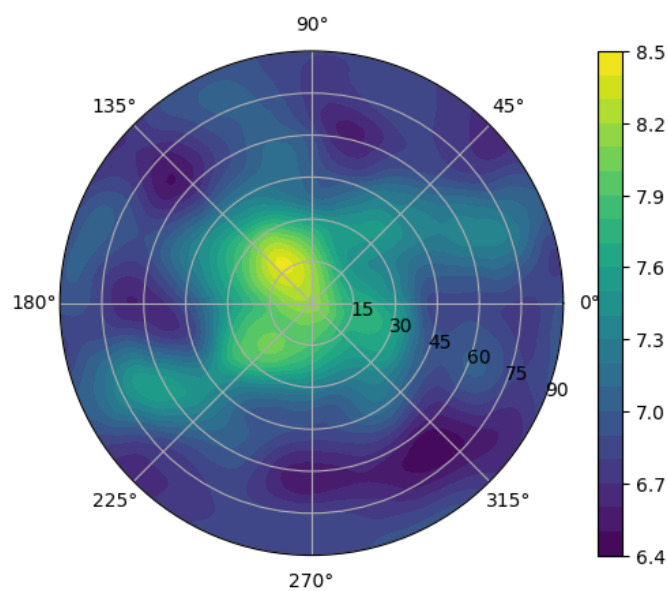
Figure 32: Directional resolution in the projection sphere.
